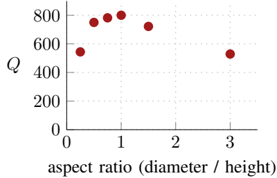
Fig. 7: Structures with a “square” aspect ratio achieve the optimum Q . To find this optimum, inductors with different aspect ratios but the same inductance and volume were simulated, and each design was optimized using the guidelines discussed in Sections III-A to III-F.
