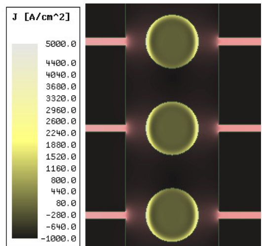
(b) Turns with multi-sided conduction
