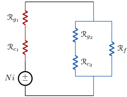
Fig. 3: Magnetic circuit model used to balance the H fields in the proposed structure by making the reluctances of the center post (red) and the return path (blue) equal. This model includes the overall fringing field outside the structure but not the gap fringing fields. The discs of core material and the quasi-distributed gaps in the center post and the outer shell are treated as lumped reluctances. The end cap reluctances are assumed to be negligible.
