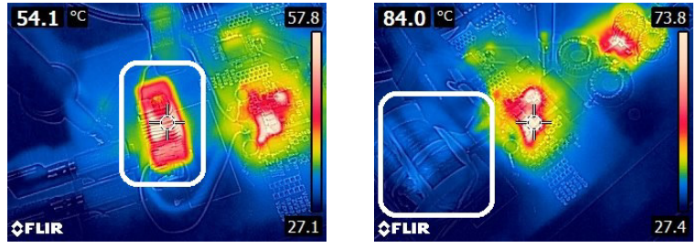
Fig. 13: Thermal images showing the proposed inductor (13b, white box) having a much smaller temperature rise for a higher converter output power than a more conventional open-magnetic-circuit inductor (13a, white box).
