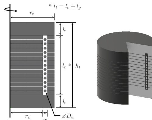
Fig. 1: Radial cross-sectional view (left) of the proposed inductor, with a center post, outer shell, and end caps enclosing a single-layer winding. Parameters defining the geometry are labelled on this view. Revolving the cross-section about the axis of rotation produces the 3D model of the inductor on the right (a piece is cut out for clarity).
