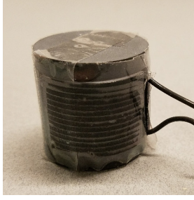
Fig. 10: Prototype inductor. Vertical windows in the outer shell were added to impede the circumferential component of flux and to allow the winding terminations to leave the structure.
