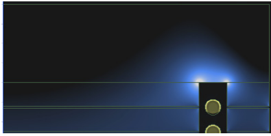
Fig. 5: Flux crowding at the end of the window leads to higher B fields (white and light blue) and thus greater core loss.
