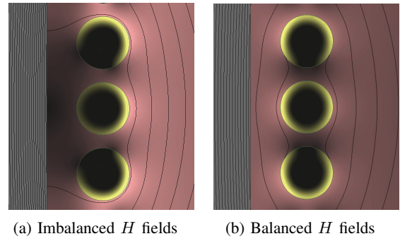
Fig. 2: When H fields (red) are balanced, the effective conduction area in the winding (yellow) is increased. For example, a winding in a high permeability rod core inductor (2a), which has a lower H field on the side of the winding near the core (grey) than away from it, has only single-sided conduction. A low permeability rod core inductor (2b) has comparable H fields on either side of the winding, so the winding has double-sided conduction. The field balance/imbalance can also be seen in the plotted B field lines. 1
