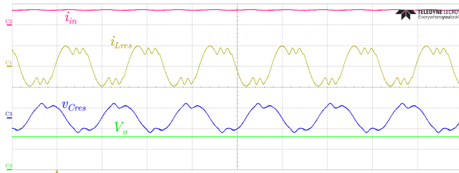
Fig. 9: Standalone operation of partial power rated charger. Key: C1 - i_{Lres} (10 A/div), C2 - i_{in} (10 A/div), C3 - v_{Cres} (200 V/div), C4 - V_o (200 V/div).
