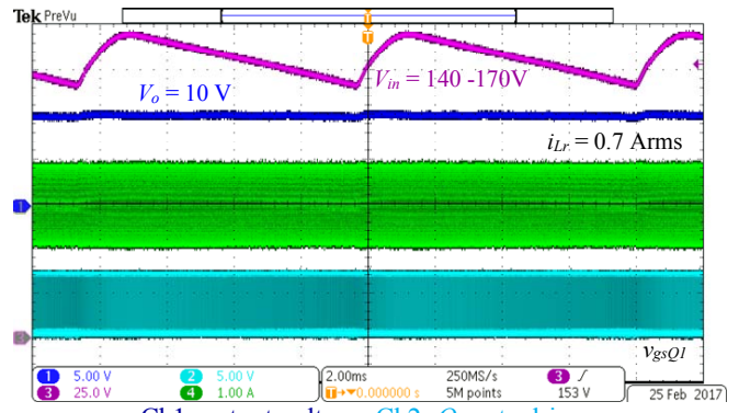
Ch1: output voltage; Ch2: Q_1 gate drive; Ch3: capacitor voltage; Ch4: resonant current Fig. 14. SRC converter with capacitor bypassing for 120 VAC with 3.3 nF capacitor and Q_3 off
