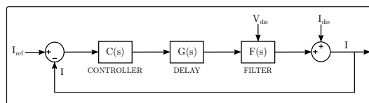
Fig. 1: A proportional resonant ( PR ) based current control structure in the abc or \alpha\beta frame [3].
