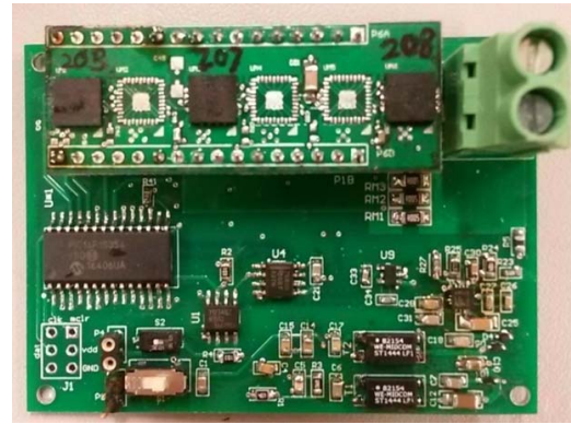
Fig.14 Three MEMS in parallel prototype.
