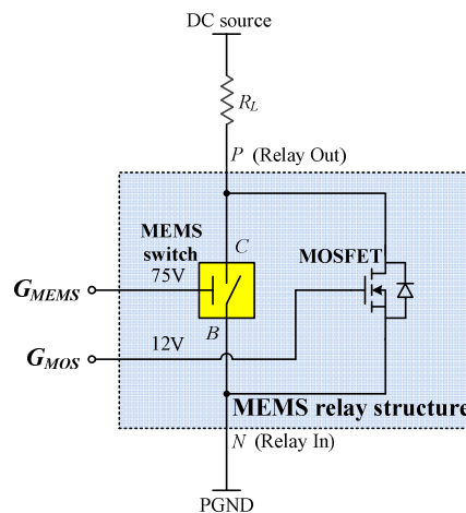
Fig.2 MEMS switch based relay with an auxiliary MOSFET.
