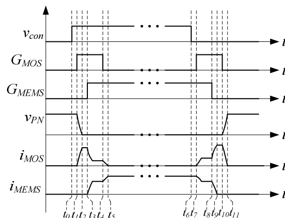
Fig.3 Operation principle of MEMS relay.
