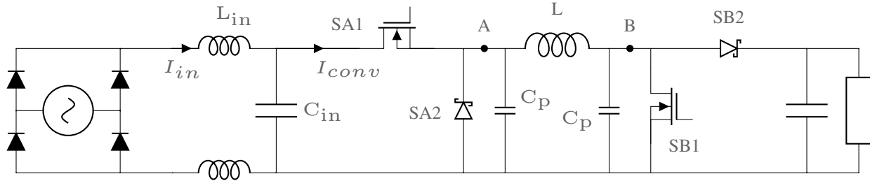
Fig. 1. The proposed power factor correction topology, which is identical to the four-switch buck-boost converter (the advantages of the proposed converter arise through control). Lumped parasitic capacitances C_p are drawn explicitly, and rectification bridge and an example emi filter are shown for completeness.
