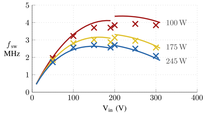
Fig. 8. Instantaneous frequencies across the rising half of the line cycle, showing reasonable frequency variation across voltage/power. Measured values agree well with curves calculated from the model in the Appendix.
