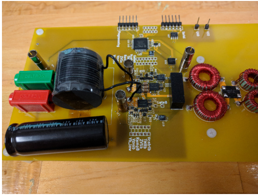
Fig. 6. Photograph of the prototype converter, including twice-line-frequency energy buffer capacitor, power stage inductor, switching and control elements, and input filter and rectifier.
