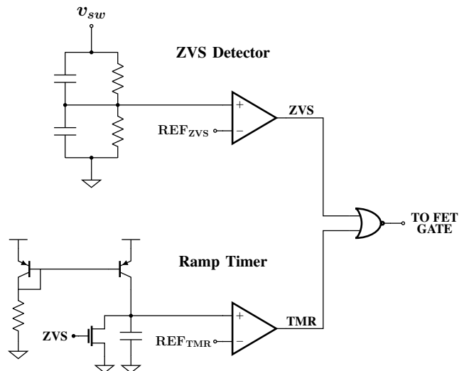
Fig. 4. Auxiliary comparator-based control circuit used for each active switch in the proposed topology, allowing for turn-on in response to zero-voltage conditions and a programmable on-time. Minor variations to this circuit may be required as discussed in Section IV.
