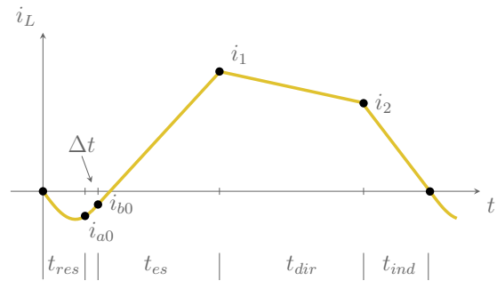
Fig. 3. High Voltage Mode inductor current waveform. This mode achieves ZVS when V_{in} < V_{out} , but is most useful where the Boost mode loses ZVS, i.e. V_{in} > V_{out}/2 . The switching cycle differs from the Boost mode primarily with the indirect delivery phase (SA2, SB2 on).
