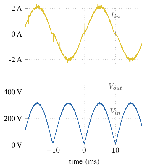
Fig. 5. Experimental operating waveforms for the proposed converter. The filtered input current has high power quality (THD < 10%), with no discernible distortion from mode transitions. Zero-crossing distortion is the major source of THD, and can be eliminated with more detailed modeling.
