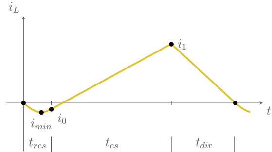
Fig. 2. Low Voltage (Boost) Mode inductor current waveform. This mode achieves ZVS when V_{in} < V_{out}/2 . The switching cycle is divided into a resonant phase (SB1, SB2 off), an energy storage phase (SB1 on), and a direct delivery phase (SB2 on).
