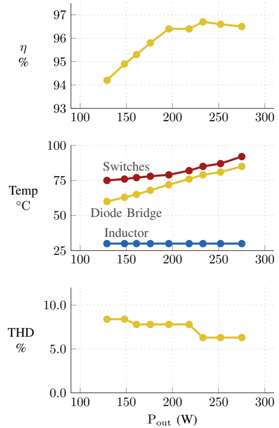
Fig. 7. Measured prototype performance, showing high efficiency and high power quality. Experiments were performed at 220 Vrms input and 400 Vdc output maintained by low-bandwidth digital closed-loop control for a resistive load. Modest forced convection was applied to the switches, though the devices used are primarily bottom-side cooled.
