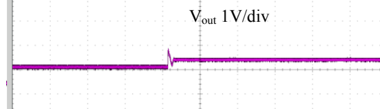
Fig. 20. Output Voltage Waveforms for Load Step of 1A to 20A
