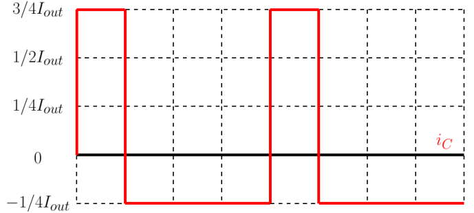
Fig. 15. Input Capacitor Current Waveforms
