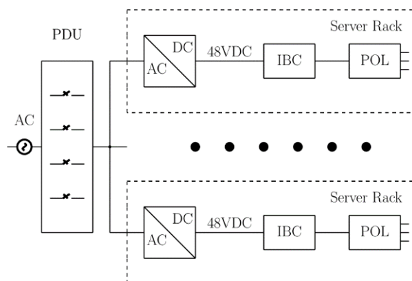
Fig. 1. Google's 48V Server Architecture “2-Stage Conversion Approach”
