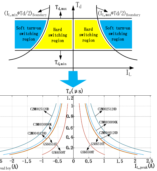
Fig. 4. The soft switching operation regions for different devices.
