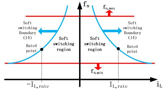
Fig. 6. The operating trajectories of MPC method.
