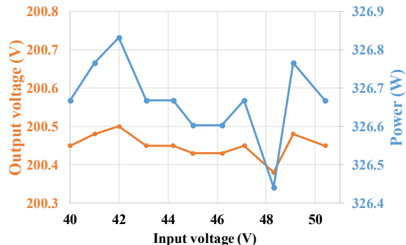
Fig. 8. Measured output voltage and power of the DAB converter under the proposed control scheme at different input voltage.
