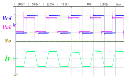
Fig. 6. Steady-state waveforms of the converter. CH1: v_{cd}=200\text{V}/\text{div} ; CH2: v_{ab}=50\text{V}/\text{div} ; CH3: v_o=10\text{V}/\text{div} ; CH4: i_L=10\text{A}/\text{div} ; Time: 5 \mu\text{s}/\text{div} .
