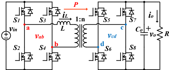
Fig. 3. DAB DC-DC converter with resistive load.
