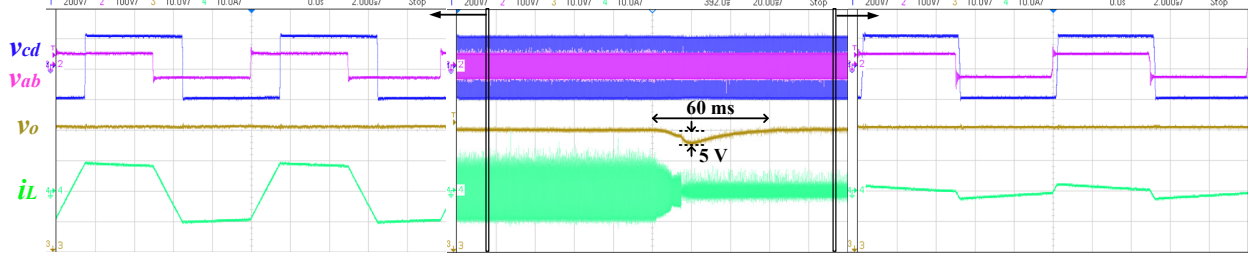
Fig. 10. The dynamic response when load changed from 324 W to 64 W and the corresponding steady-state waveforms.
