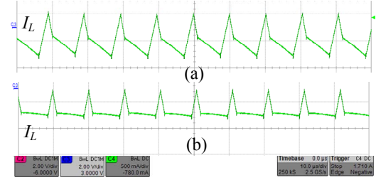
Fig. 12. Enhanced-boost mode, V_{out}=3.3V (a) V_{in}=2.8V (b) V_{in}=3.2V .
