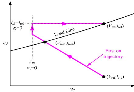
Fig. 7. Illustrative movement of the state plane for the voltage-deviation and current-constrained mode handling a loading transient.
