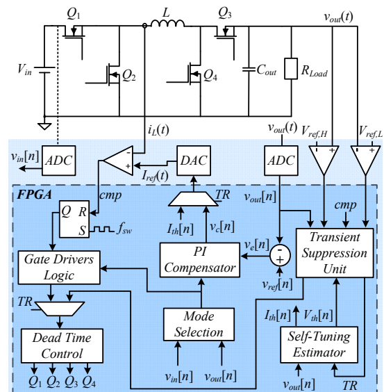
Fig. 1. Simplified schematic diagram of a non-inverting buck-boost converter with current-programmed controller.
