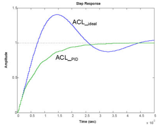
Fig. A1. Step responses of closed-loop system compensated with ideal controller and derived compensator, for closed-loop specifications of slow rise time and high overshoot.
